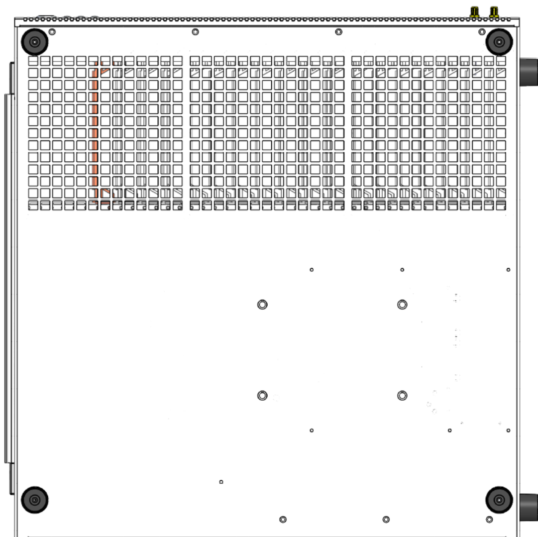
Figure 12 Bottom View
