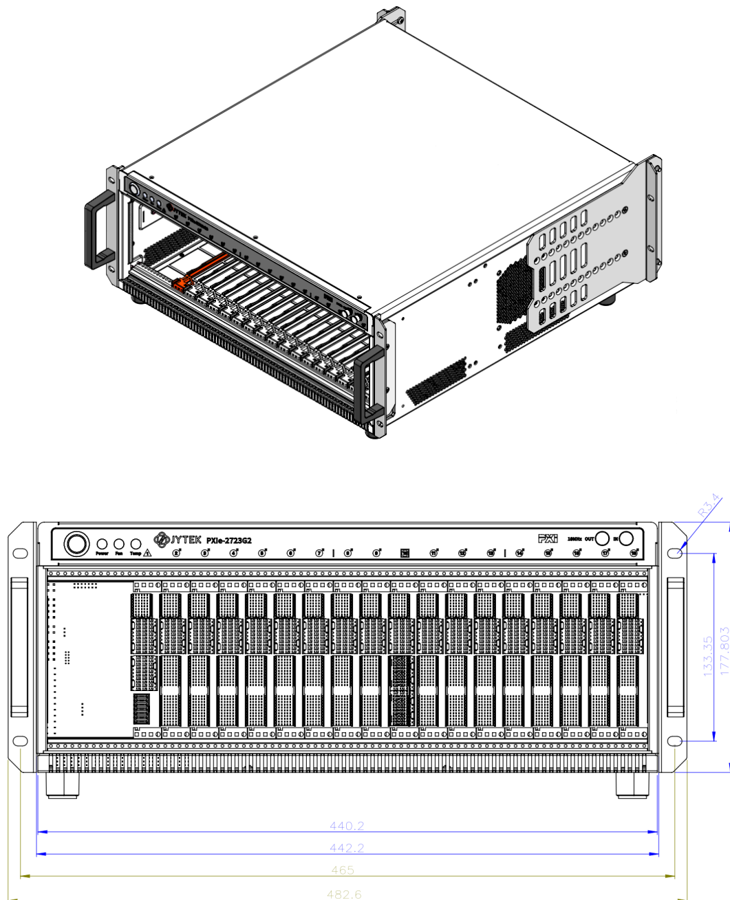
Figure 40 PXIe-2723 rack mount kits dimension
