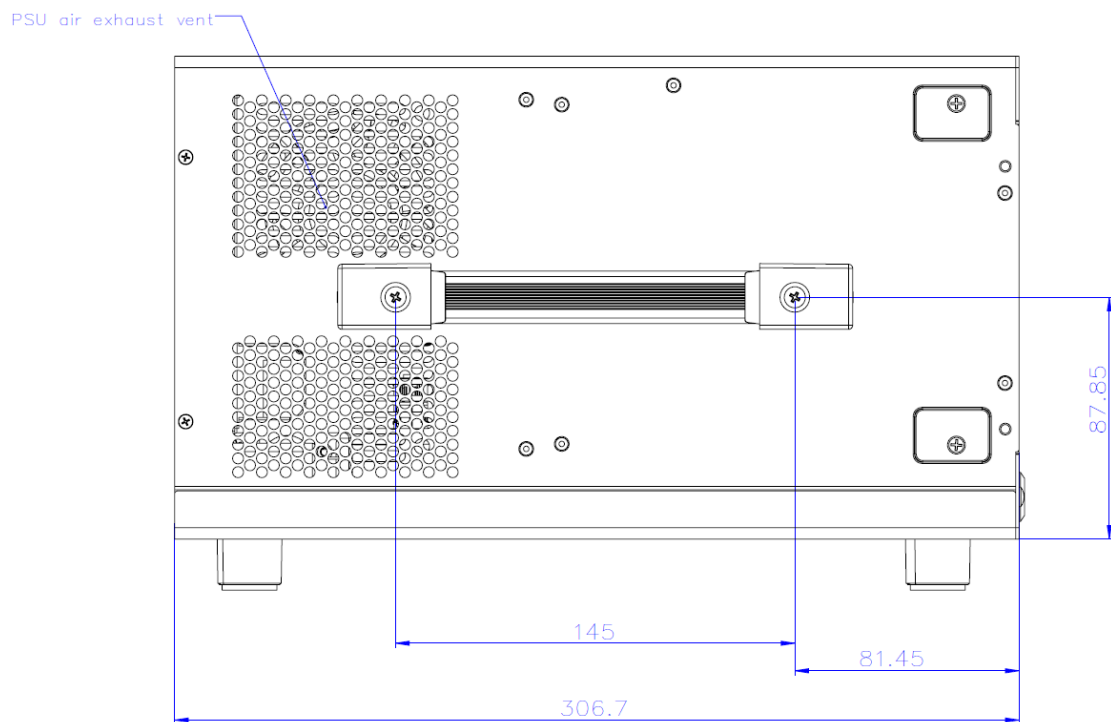
Figure 4 Left Side View (PXIe-2519 Gen 3/Gen 2/DC)
