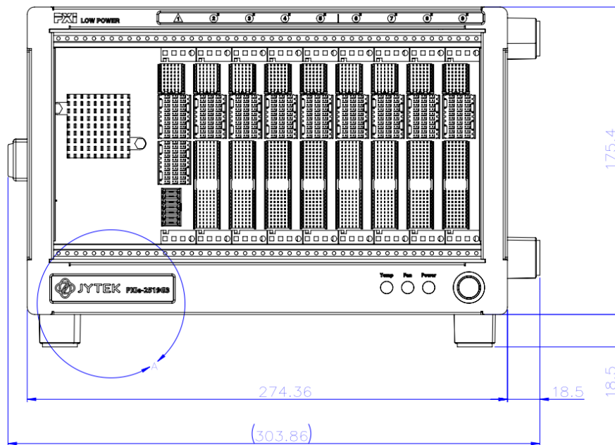
Figure 3 Front View (PXIe-2519 Gen 3/Gen 2/DC)
