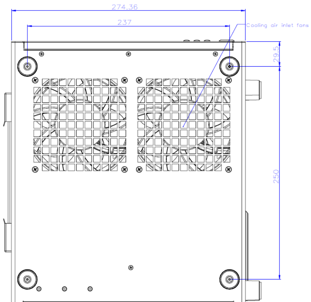
Figure 8 Bottom View (PXle-2519 Gen 3/Gen 2/DC)
