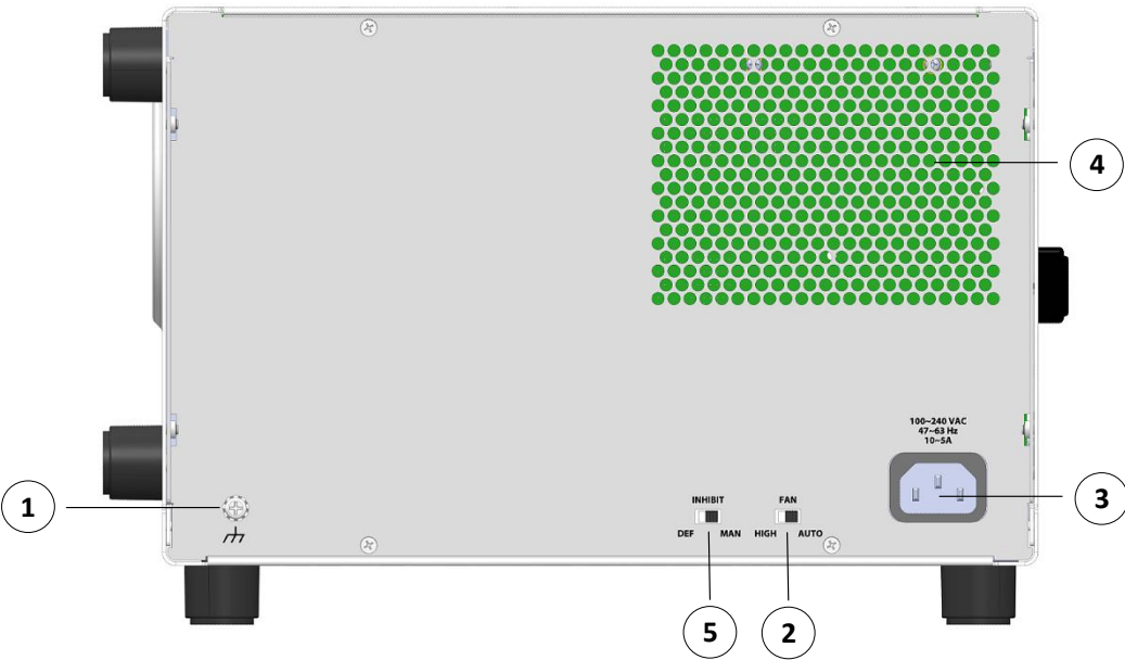
Figure 12 PXle-2519G2/G3 Rear Panel
