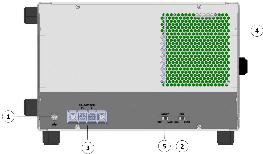
Figure 13 PXle-2519DC Rear Panel
