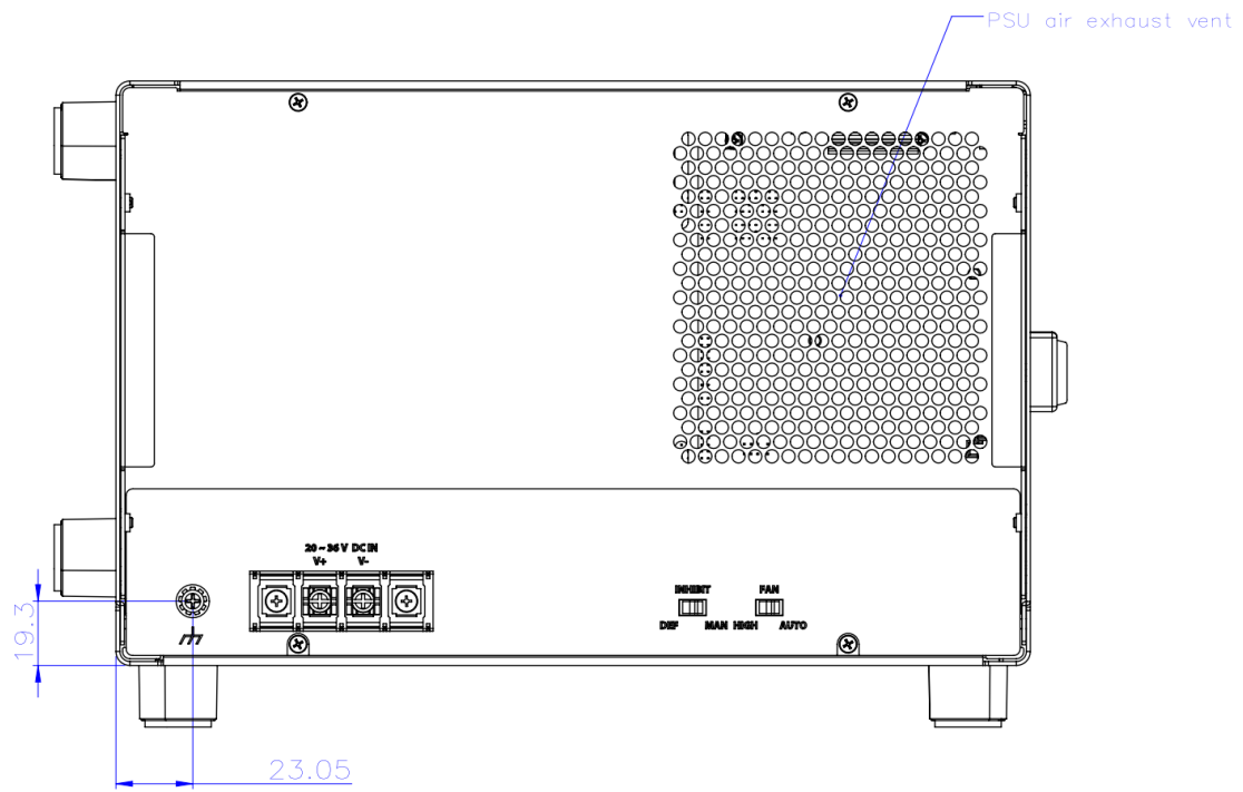
Figure 9 PXle-2519DC Rear View
