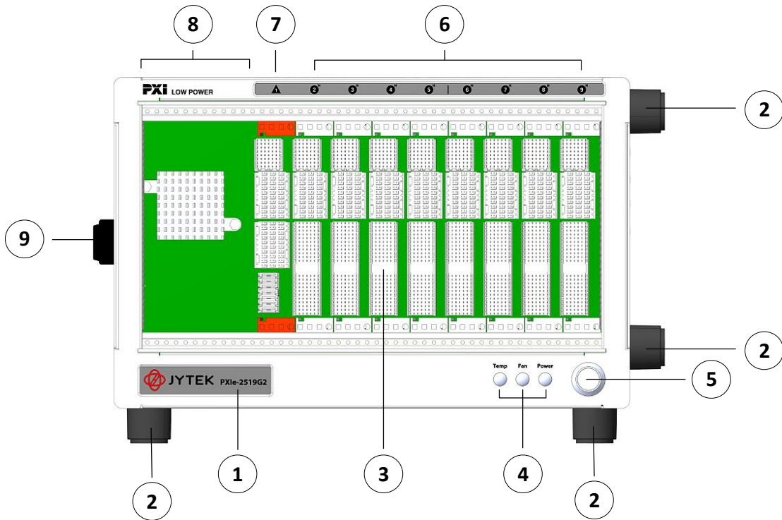
Figure 11 Front Panel
