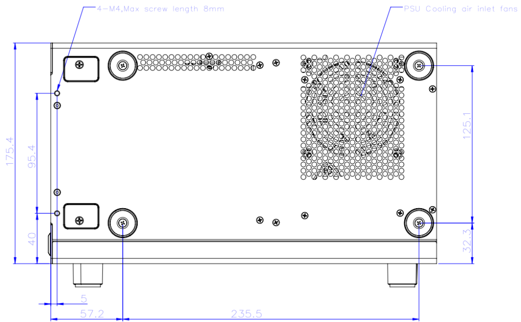
Figure 5 Right Side View (PXle-2519 Gen 3/Gen 2/DC)
