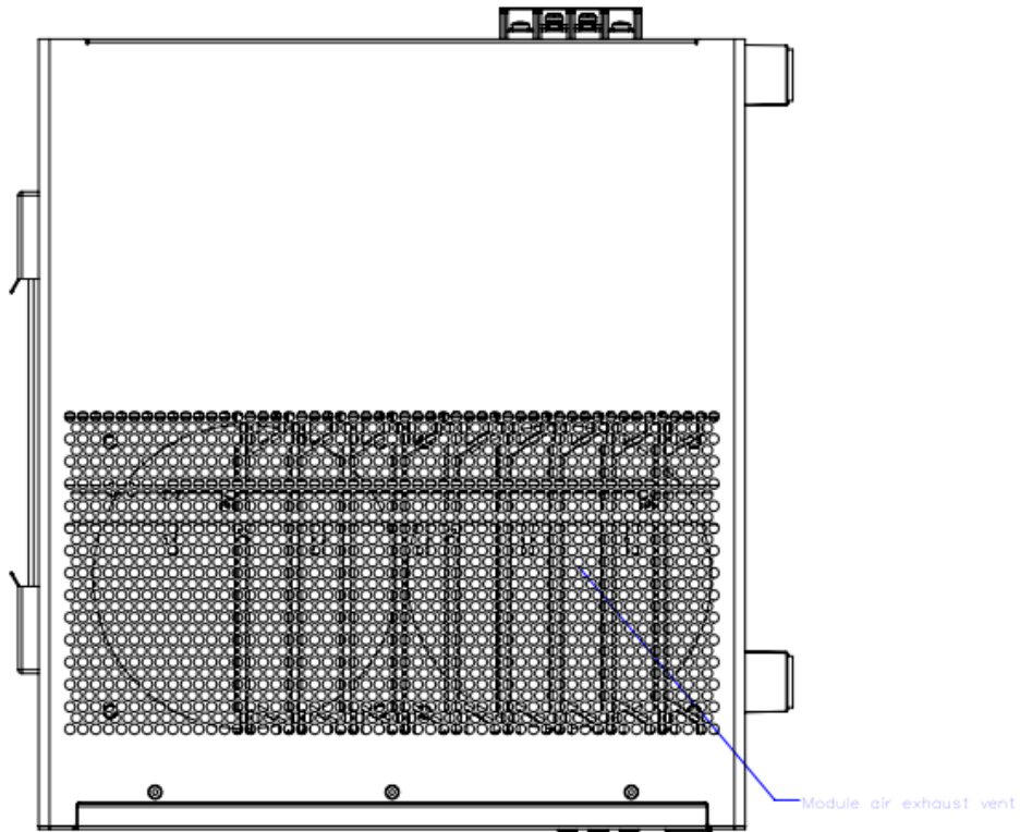
Figure 10 PXle-2519DC Top View
